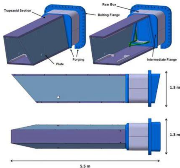
Figure 2. Upper Port Plug structure and general dimensions.
