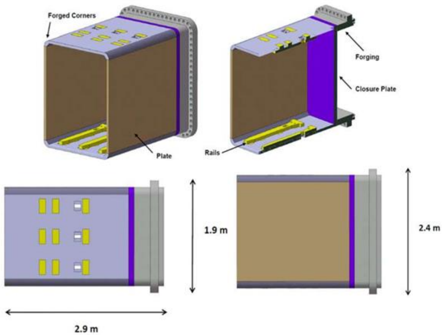
Figure 3. Equatorial Port Plug structure and general dimensions.
